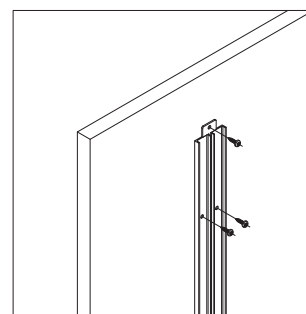
4 Screw fixing of M19 and end cap
