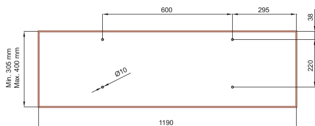
300-mm shelf bracket ( LTTAB30B ) and folded / side-hung bracket ( LTBPTABB )
